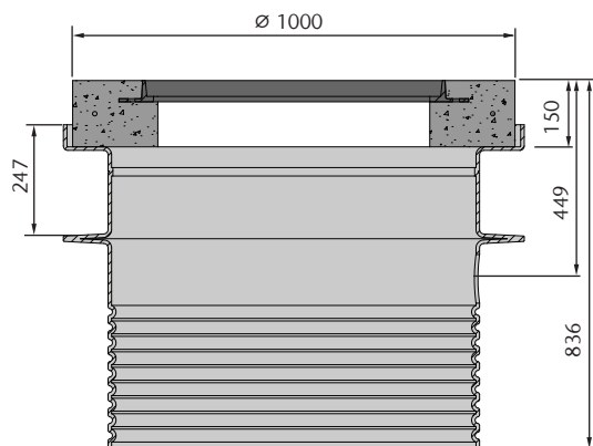
Cover, collar and riser tube
